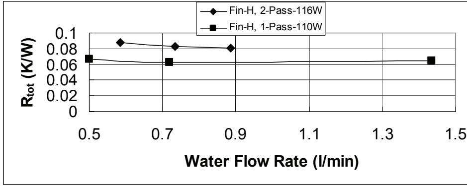
Figure 4. R_{tot} of 1-pass vs. 2-pass micro-channel coolers.
