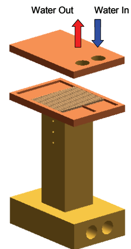
Figure 3. a) Prototype test sample of 1-pass micro-channel cooler with 20 mm micro-channel flow length, b) Test setup illustrated for a 2-pass design.
