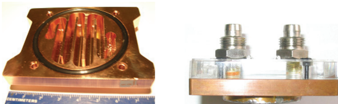
Figure 1 a) Thermaltake “Bigwater” waterblock having one serpentine channel 4.5 mm wide x 10 mm deep, b) Side view with Plexiglas cover and fluid connectors.
