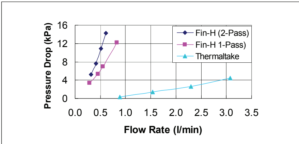
Figure 5. Measured pressure drop for the 1-pass and 2-pass micro-channel design and for the Figure 1 Thermaltake “waterblock.”
