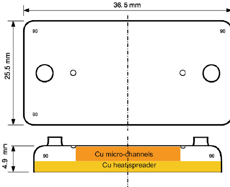
Figure 8. Illustration of fabricated micro-channel cooler.
