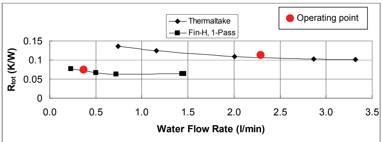
Figure 6. Comparison of R_{tot} for 1-pass micro-channel cooler and Thermaltake cooler.
