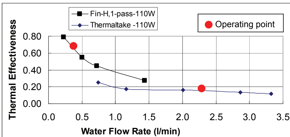
Figure 7. Thermal effectiveness vs. water flow rate for micro-channel cooler vs. Thermaltake.
